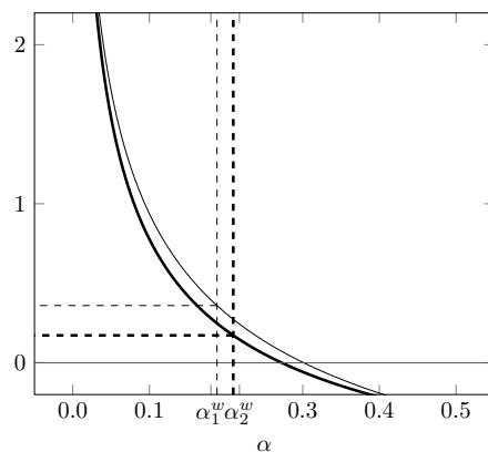
Figure 11: \beta_{\alpha a}(\alpha, a) for a = 0.2 (thin curve) and a = 0.3 (thick curve)
